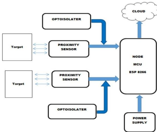
Fig. 1. Block Diagram of Implemented System count and display
