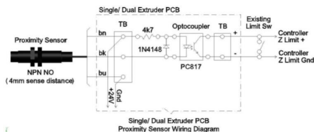
Fig. 3 . Circuit diagram of System Implemented
