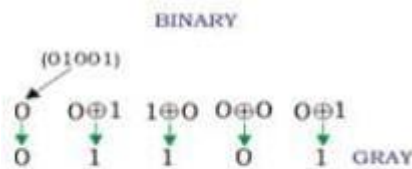
Figure 7: Binary to gray conversion
