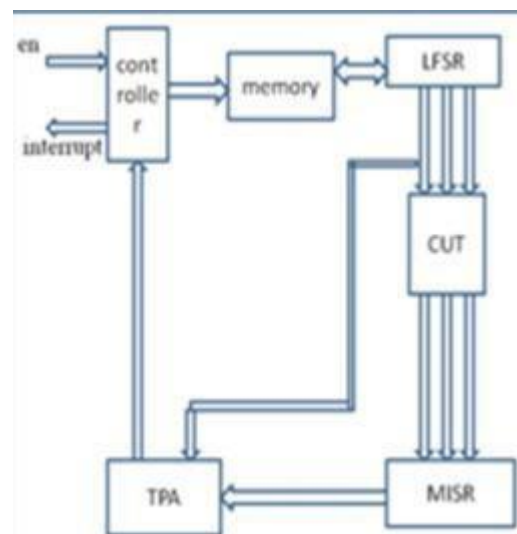
Figure 1: ATPG system on-chip circuit
