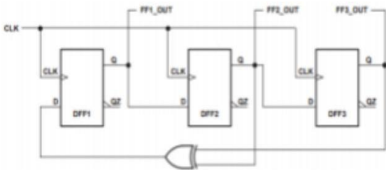
Figure 2: LFSR Circuit Exclusive-OR gate
