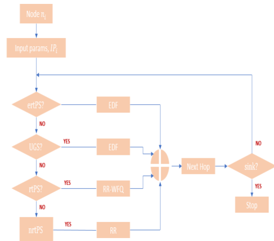
Fig 4.2: Flow Diagram of WiGrid in Smart Grid Communication
