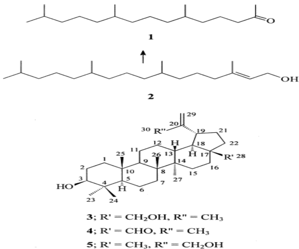
Figure 2: Lupane triterpenoid structure
