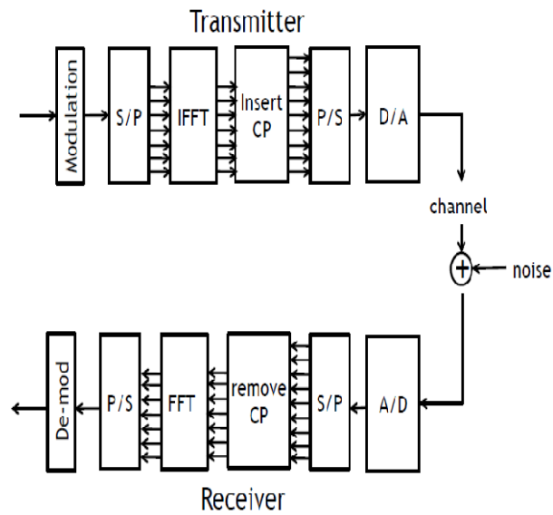
Figure.2 OFDM system block diagram
