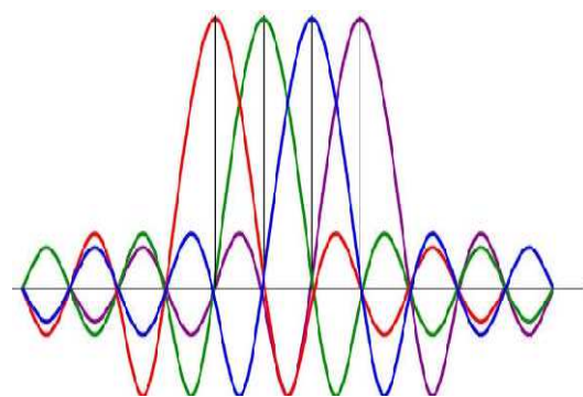
Figure.1 OFDM spectrum
