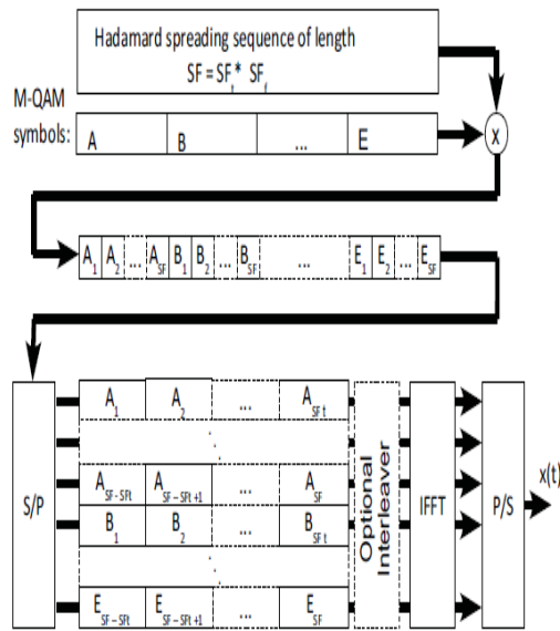
Figure.4 Scheme of 2D spreading in OVS-OFCDM
