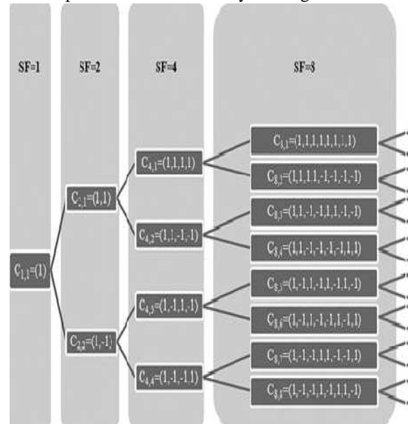
Figure.6 1D OVSF Codes Tree
