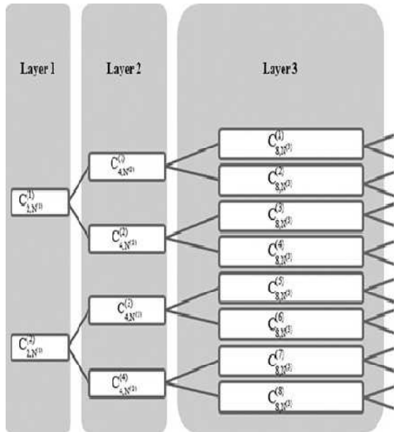
Figure.7 2D OVFS Codes Tree
