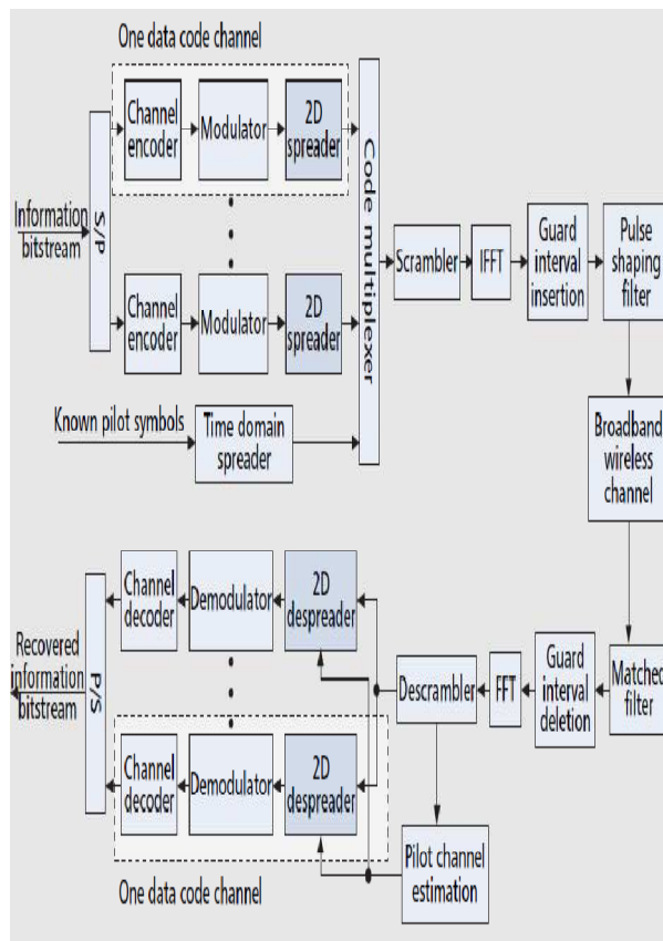
Figure.3 OFCDM system block diagram
