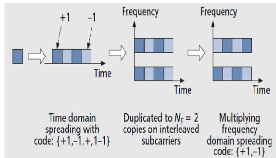
Figure.5 2D spreading with 1D OVSF Code
