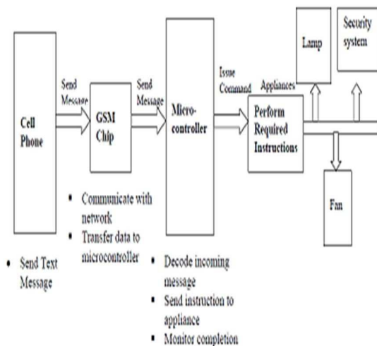
Figure2: Block Diagram of home Automation System
