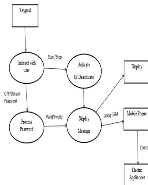
Figure1: Data Flow Diagram of System.
