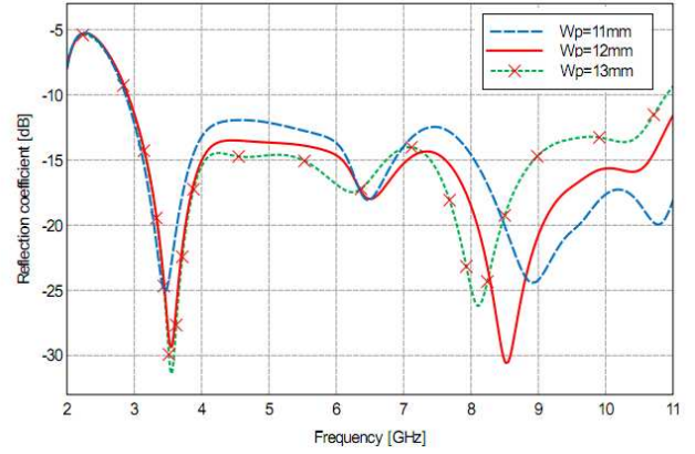
Fig.6 Return loss vs. frequency graph for different width of patch
